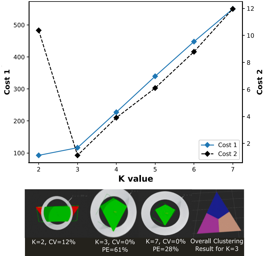
Fig. 6. Comparison of two cost functions for different values of K in K-means segmentation of a triangle-shaped planar patch. The bounding-box-based cost function is represented as cost 1 and the point-based cost function is represented as cost 2.
